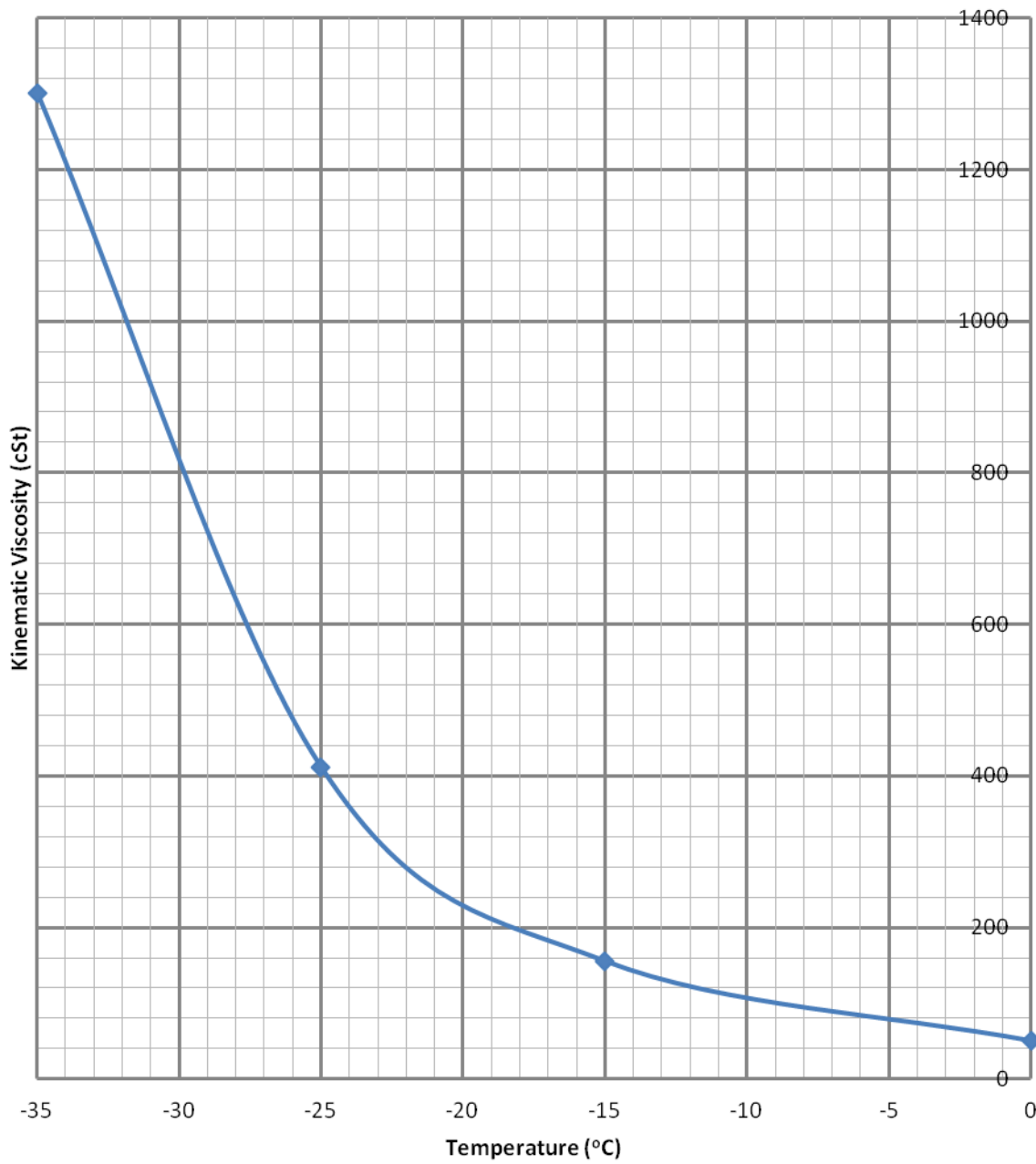
Kinematic Viscosity Curve for Scavex
